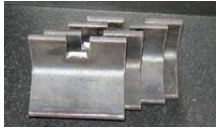
1" X 1" X 1/8" angle, with a 10mm wide slot in one side, 15mm deep
