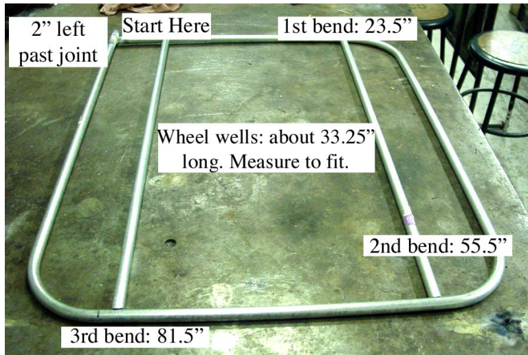
Bending diagram and sequence for the mainframe. Add the wheelwells after the mainframe is made, cut to fit each side.
